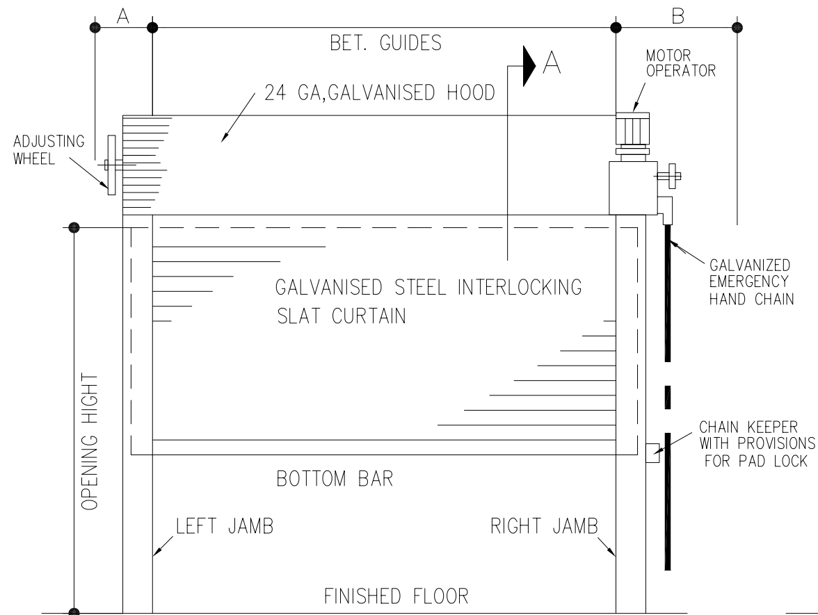
INSIDE ELEVATION RIGHT HAND AS SHOWN LEFT HAND OPPOSITE OF SHOWN
