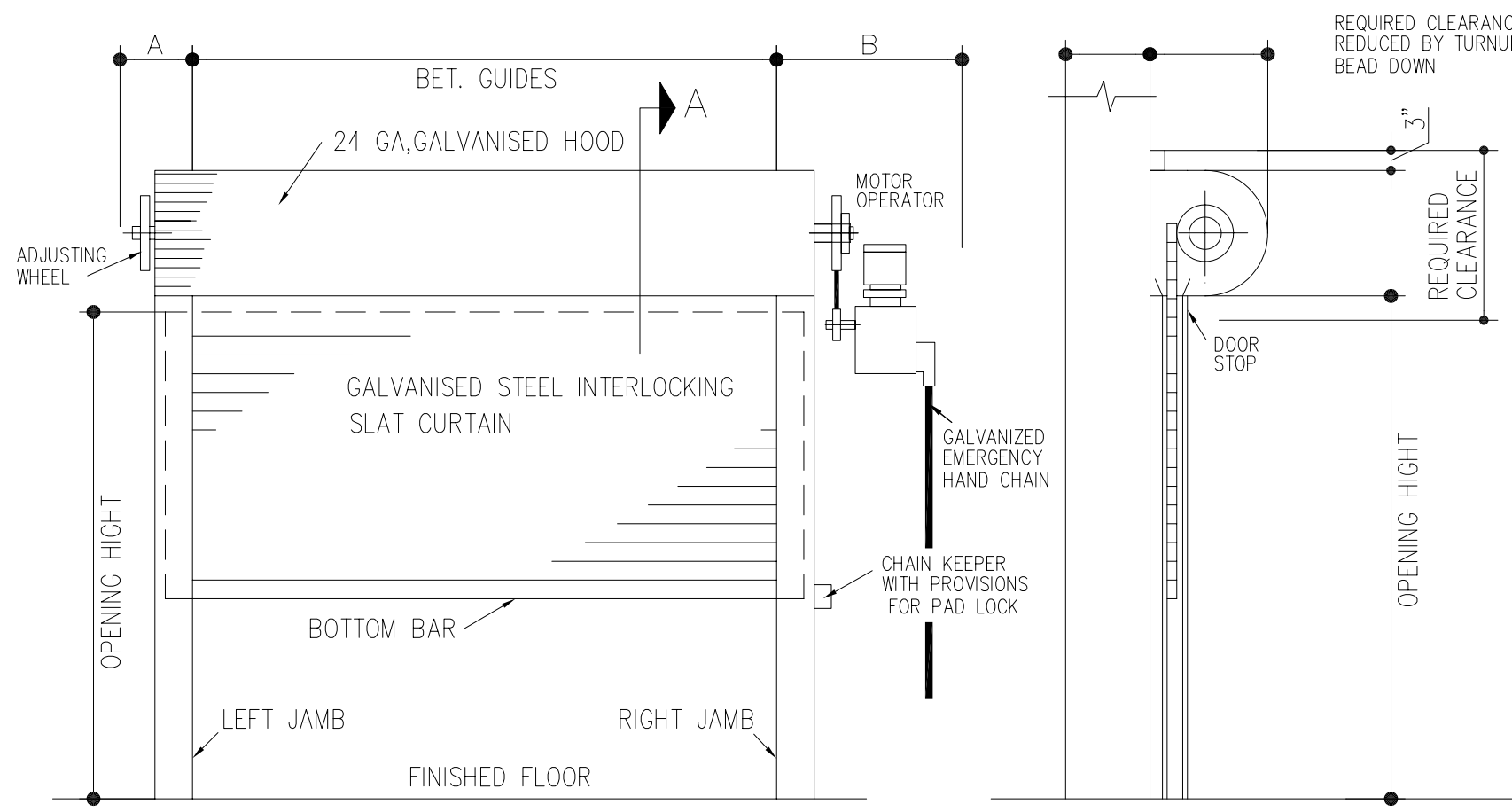
INSIDE ELEVATION RIGHT HAND AS SHOWN LEFT HAND OPPOSITE OF SHOWN
